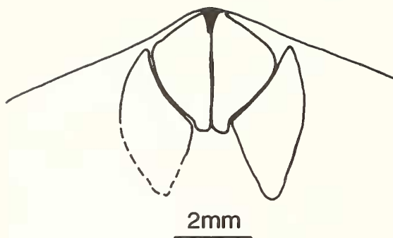
TEXT-FIG. 9. Adductor muscle scars in the brachial valve (see Pl. 1, fig. 12).
